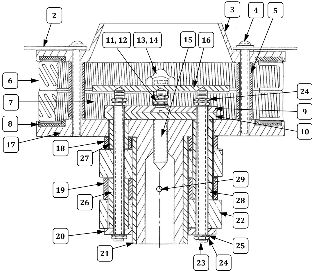
Model 3005EDX 7" Spinner Head Complete
